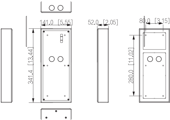
Dimensions (mm[inch])
