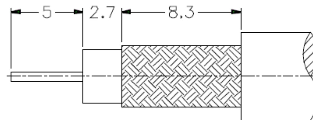
RECOMMENDED CABLE STRIPPING DIM'S
