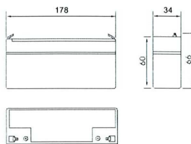
Outer dimensions (mm)
