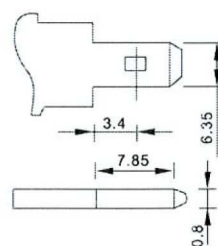
Terminal Type (mm)
